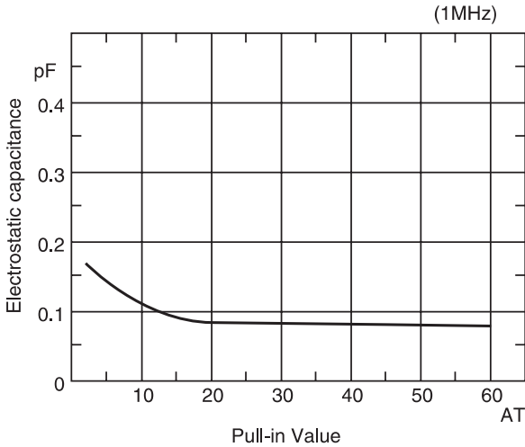
(5) Electrostatic capacitance
