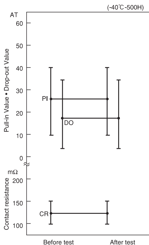
(5) Low temperature storage test
