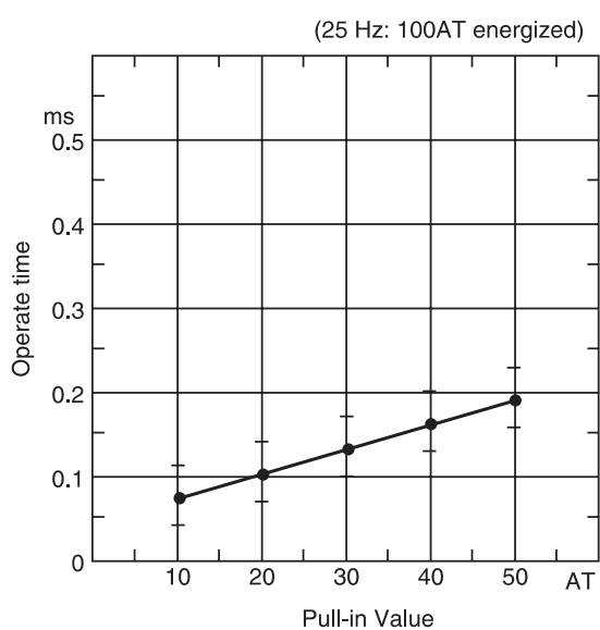
(1) Operate time
