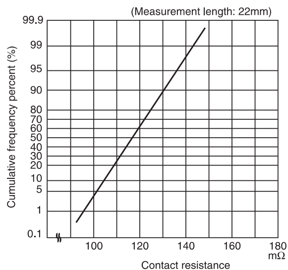
(2) Contact resistance
