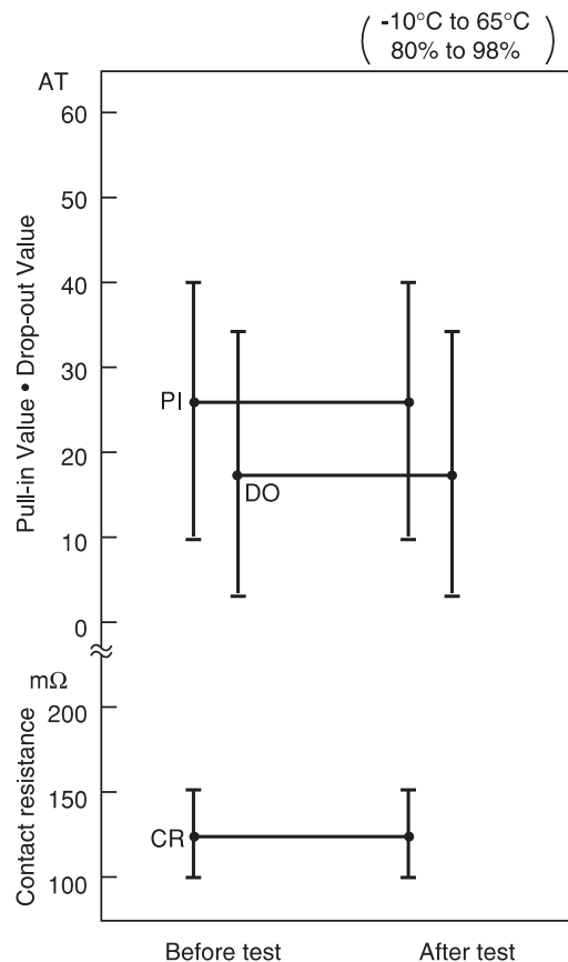
(3) Temperature and humidity cycle
