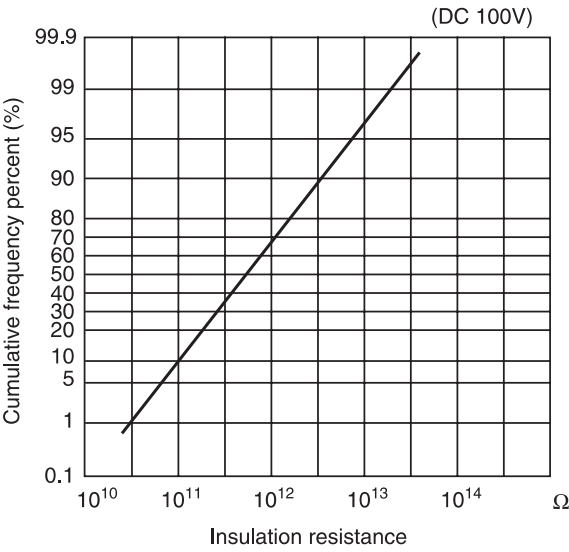
(4) Insulation resistance
