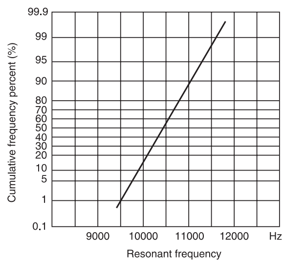
(4) Resonant frequency
